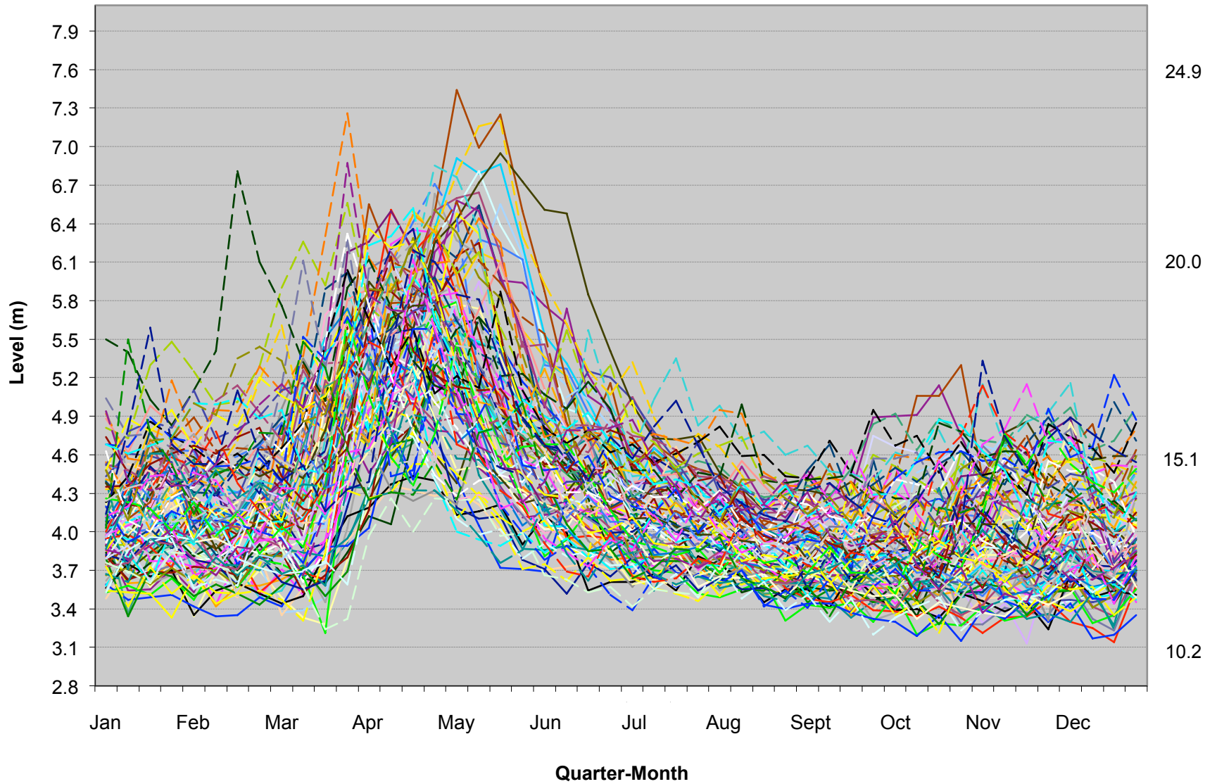
Plan Bv7 2011 Lac St. Pierre Levels for All 101 Years
